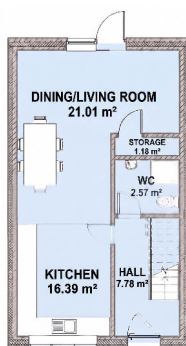
Ground Floor
